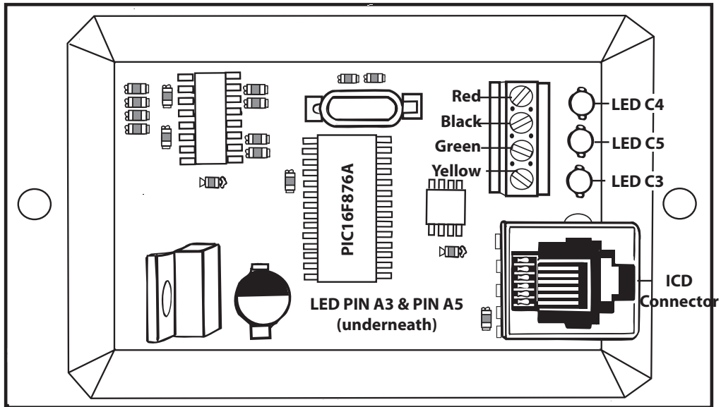
RFID Board
